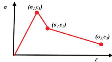
Fig. 12 The shape of tensile \sigma - \epsilon relationship
