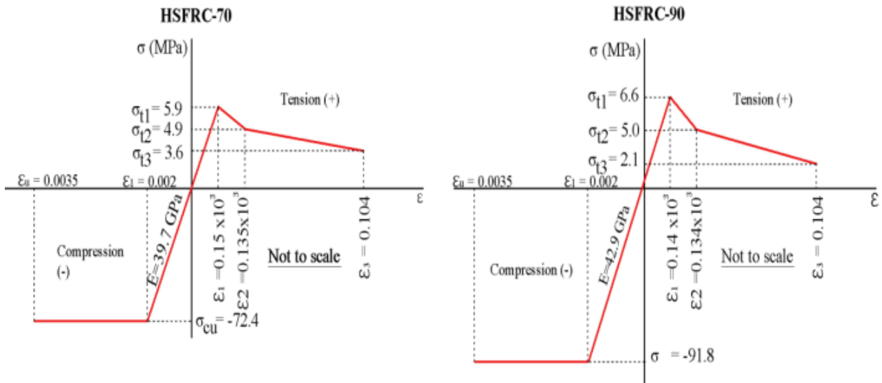
Fig. 4 The first estimate of the \sigma - \epsilon relationship for HSFRC according to [3]
