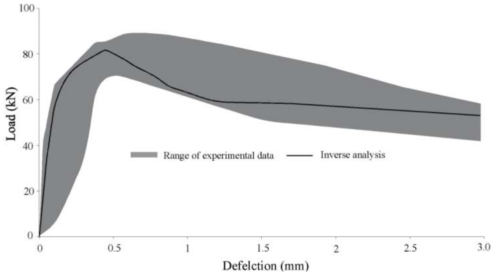
Fig. 10 Measured and calculated P- \delta behaviors: Proposed \sigma - \epsilon relationship-HSFRC-90
