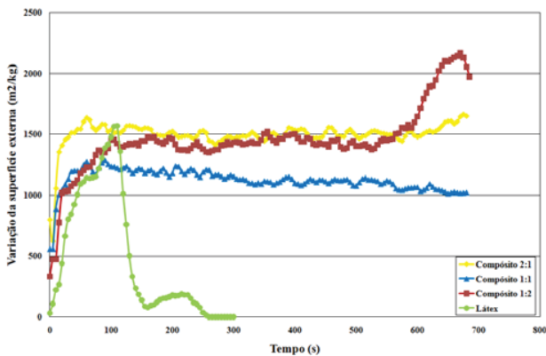
Fig. 16 Comparison of the external surface variation in function of time
