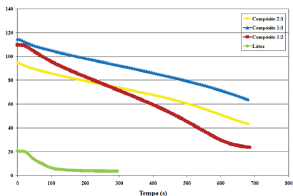
Fig. 20 Comparison of weight loss versus time
