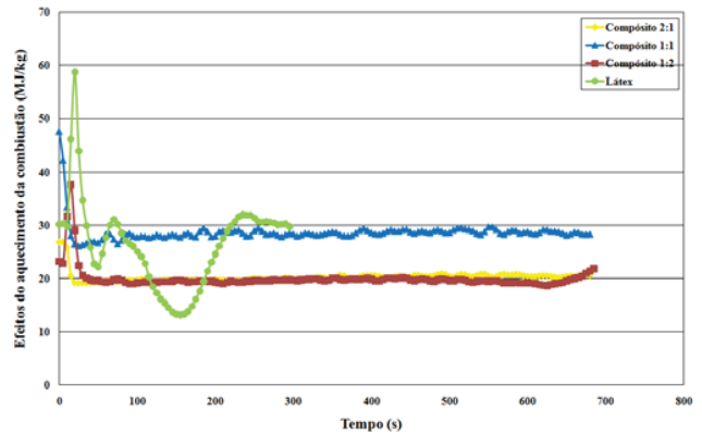
Fig. 17 Comparison of the effect of the heat of combustion as a function of time
