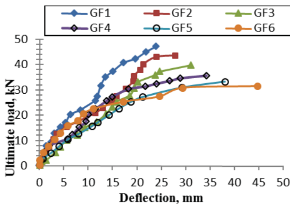
Fig. 6 Load against deflection, at mid-span
