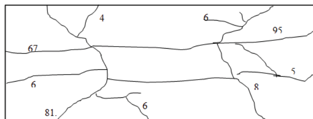
(b) Typical crack pattern for panel as two-way slab – bottom wythe
