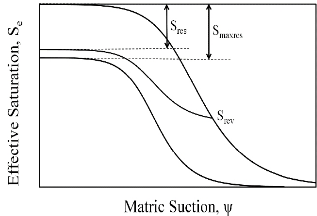
Fig. 2 Theoretical scanning loops of a hypothetical apparent saturation curve
