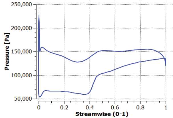
Fig. 10 Blade loading at 5 degree flow orientation
