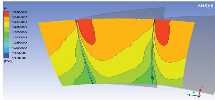
Fig. 17 Pressure contours at Blade TE (Normal flow)
