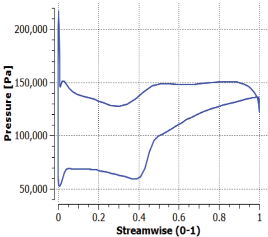
Fig. 9 Blade loading at clean flow
