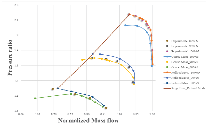
Fig. 6 Mesh study and CFD model validation
