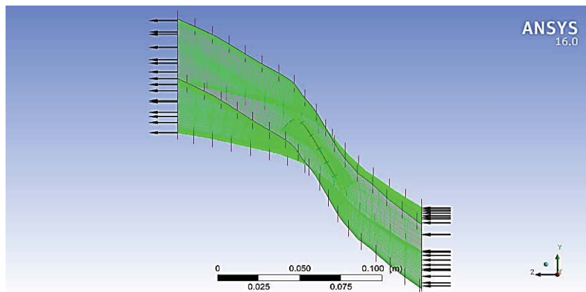
Fig. 5 Flow direction in blade passage (Inlet & Outlet)
