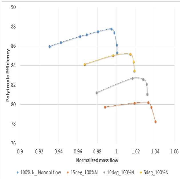
Fig. 8 Polytropic efficiency of distorted flows at 100%N
