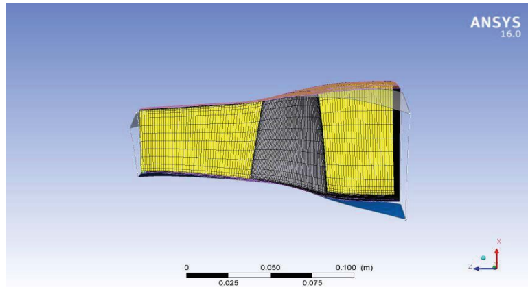
Fig. 4 Single passage (Hub, Blade & Shroud)
