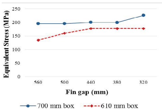
Fig. 14 Relationship between fin gap and equivalent stress
