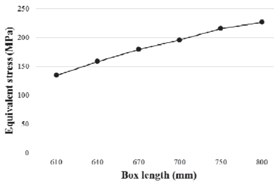
Fig. 13 Relationship between box length and equivalent stress
