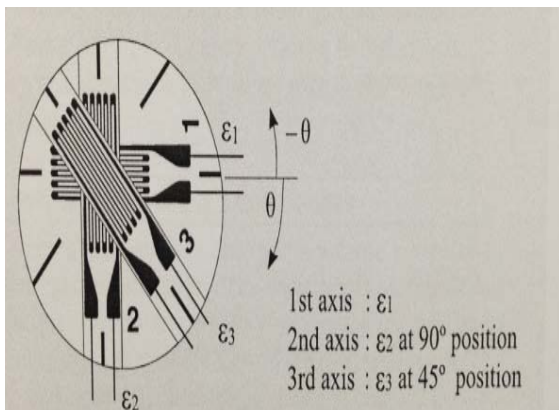
Fig. 4 Strain gages in 45°-rectangular rosette orientation
