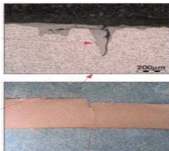
Fig. 2 Microscopic examination of the crack
