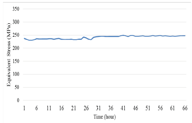
Fig. 10 Equivalent stress during operation at full capacity
