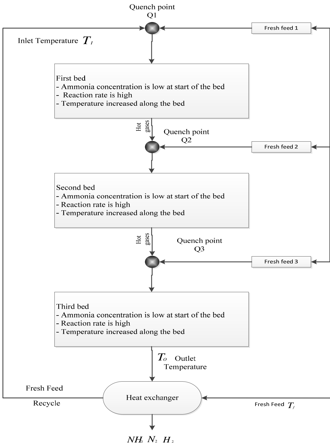
Fig. 1 Schematic representation of the ammonia fixed-bed reactor
