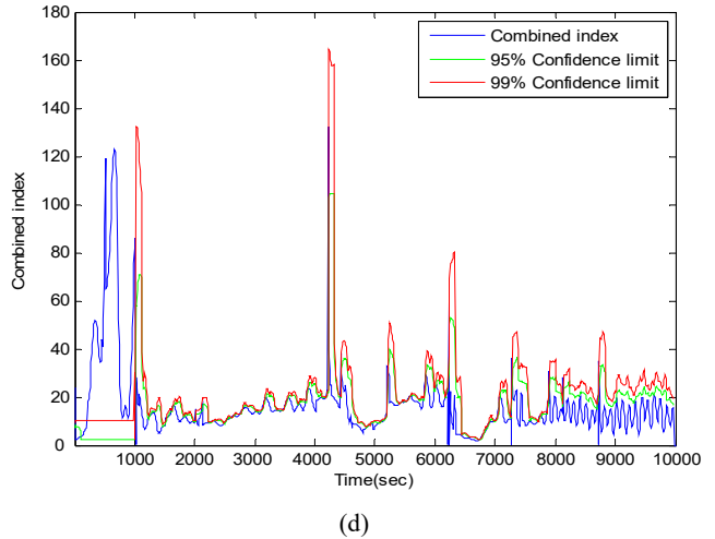
Fig. 7 (a) Hotelling T^2 for RADPLS on test data (fault100 samples), (b) SPEx for RADPLS on test data (fault100 samples), (c) SPEy for RADPLS on test data (fault 100 samples), (d) Combined index for RADPLS on test data (fault 100 samples)
