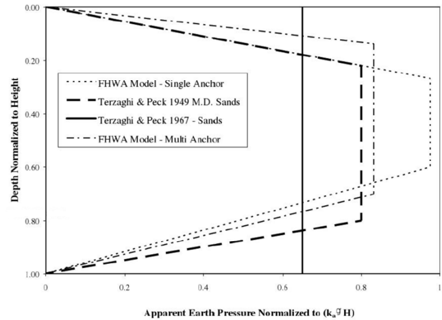
Fig. 5 Apparent earth pressure diagrams [5]
