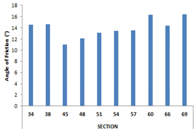
Fig. 9 Analyzed values of the angle of Friction
