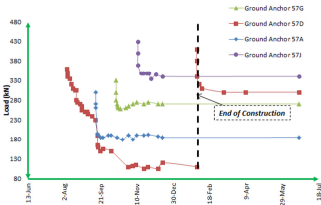
Fig. 4 Curve load vs time of the section 57
