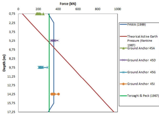
Fig. 7 Load measurements for section 45
