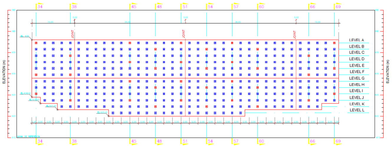
Fig. 1 Geometry of anchored wall
