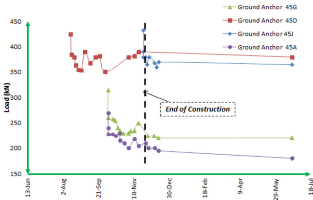
Fig. 3 Curve load vs time of the section 45
