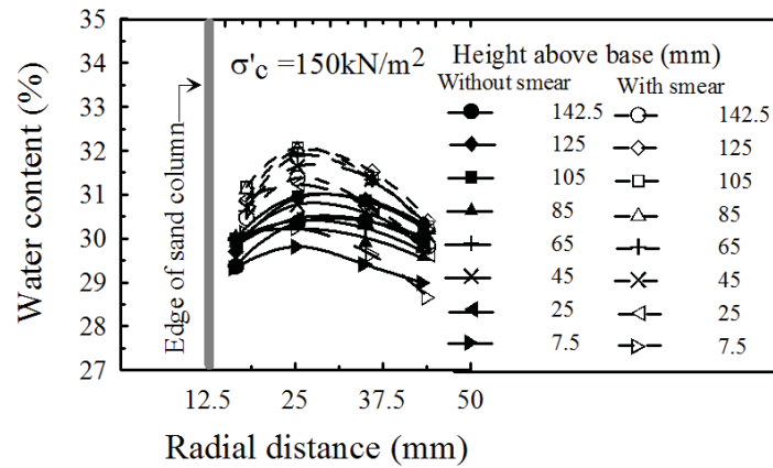
(a) Mean eff. stress -150kPa
