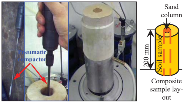
Fig. 4 Compaction of SCP in reconstituted clay specimen
