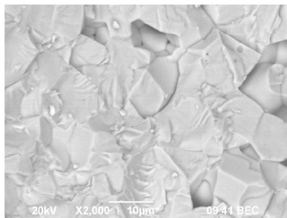
Fig. 4 SEM micrograph of the cross-section of ceramics \text{LaNb}_{0.9}\text{W}_{0.1}\text{O}_{4.05} sintered at 1673 K
