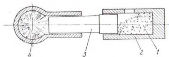
Fig. 1 Scheme of explosion press for metal chips briquetting: 1- filled chips; 2- container; 3- punch; 4- explosion chamber
