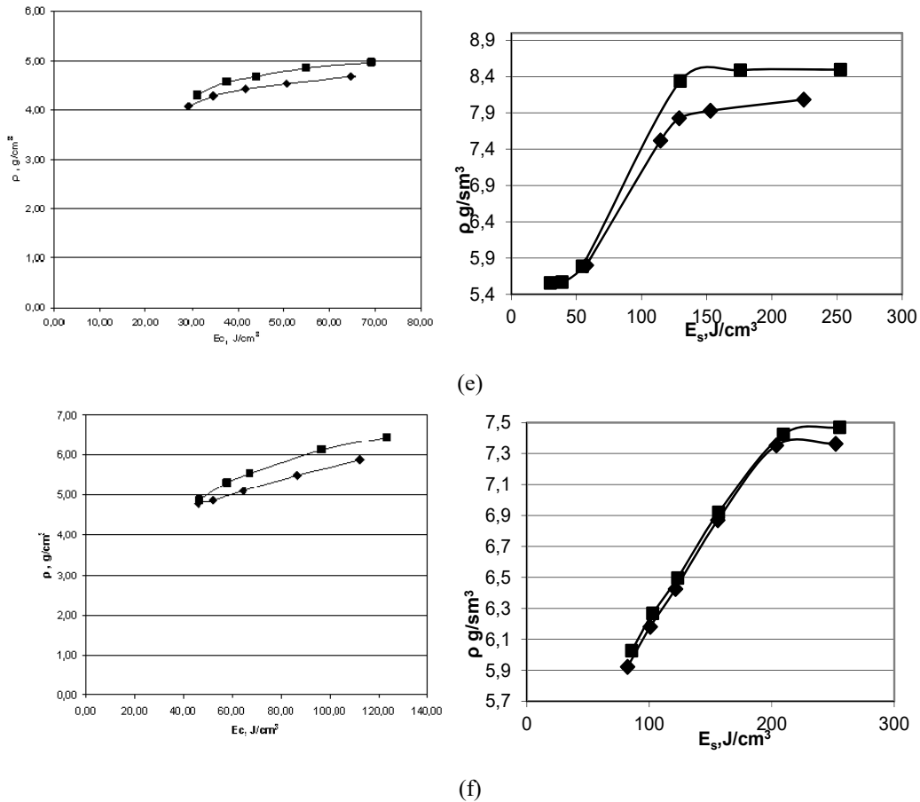
Fig. 4 Results of impact briquetting with different impact velocities V_i ; left- V_i = 4.10-5.32 m/s; right V_i = 6.9-7.16 m/s [7] a) Armco iron; b) steel; c) gray cast iron; d) aluminum alloy; e) pure cooper; f) brass
