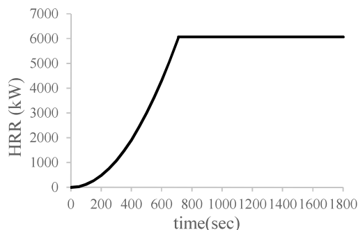
Fig. 4 Heat release rate curve
