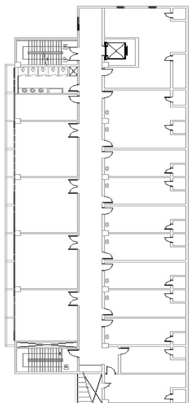
Fig. 1 Floor plan
