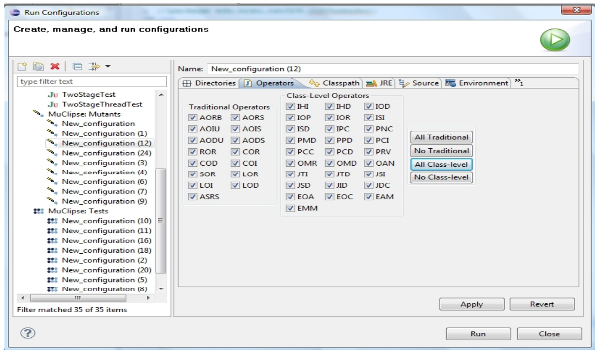
Fig. 2 MuJava Mutation Operators
