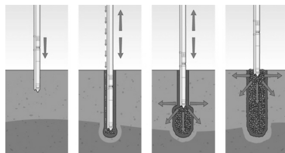
Fig. 1 Vibro displacement by dry bottom-feeding method, [16]
