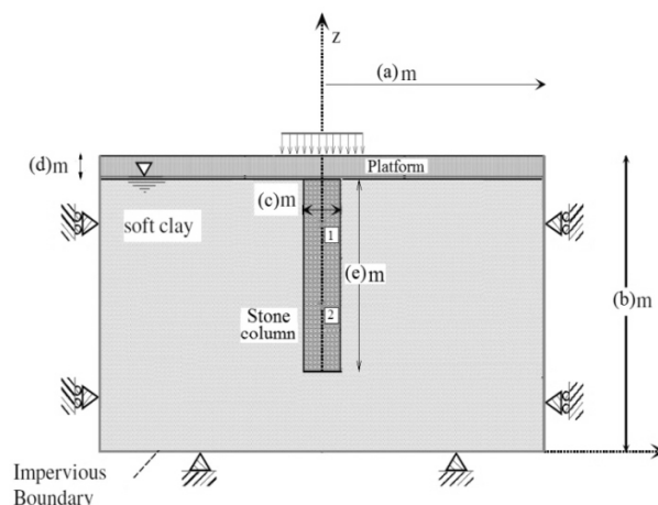
Fig. 3 Boundary conditions in studied model
