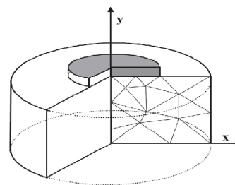
Fig. 2 Axisymmetric problem. [25]
