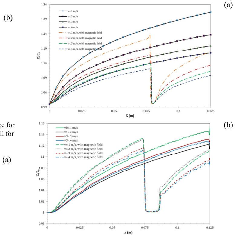
Fig. 6 Magnetic field effect on the LSC along the wall for different Re number; (a) In the lumen-tissue interface, (b) The upper layer of porous domain
