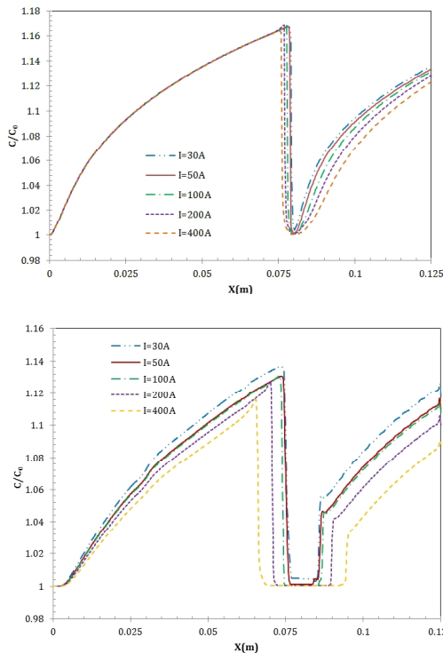
Fig. 5 Behavior of LSC in the presence of a magnetic field by different wire intensity in the lumen-tissue interface (a) and upper layer of porous domain (b)
