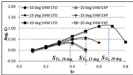
Fig. 6 Time averaged C_T for different S_T with varied \alpha_0 (namely 10, 15 and 20 degs), where the vertical dotted lines represent S_{Tc} . The comparison between experiment and numerical results are also shown
