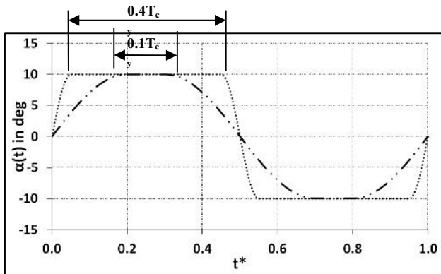
Fig. 3 Different trapezoid base length followed in the present study
