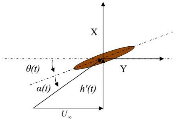
Fig. 2 Schematic drawing showing the effective angle of attack \alpha(t) seen by an observer travelling with the pivot point of the airfoil
