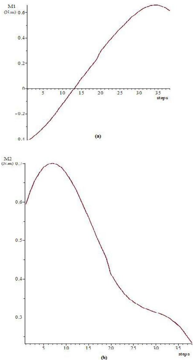
Fig. 10 Values of M_1 , M_2 for the first day of the year respectively
