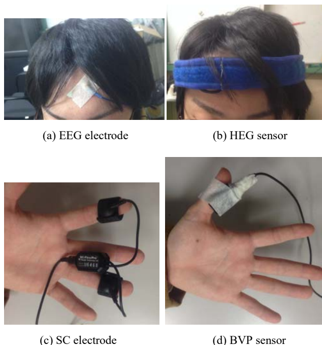
Fig. 2 Physiological sensors
