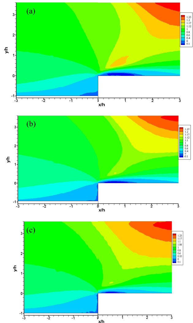
Fig. 2 Contour plots of streamwise mean velocity in the recirculation region for (a) SM, (b) SP and (c) SG
