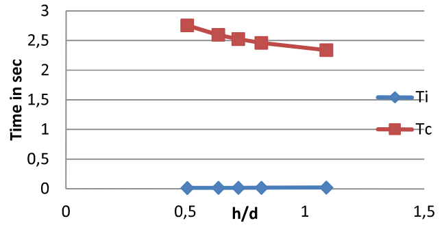
Fig. 7 Variation of Impulsive and Convective Time Period with h/d (100 KL)
