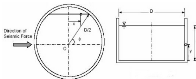
Fig. 2 Plan and Sectional Elevation of Tank [9]
