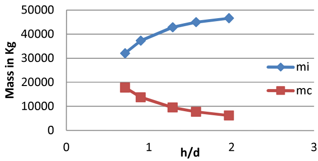
Fig. 3 Variation of Impulsive and Convective Mass with h/d (50 KL)
