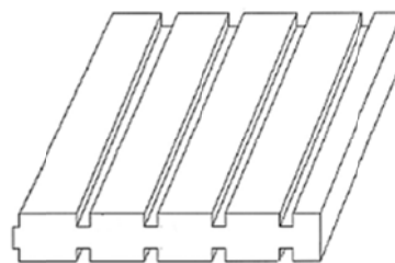
Fig. 2 Two sets of parallel channels in counterflow [13]
