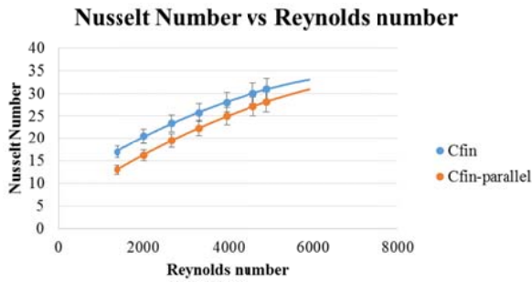
Fig. 20 Variation of Nusselt number with Reynolds number
