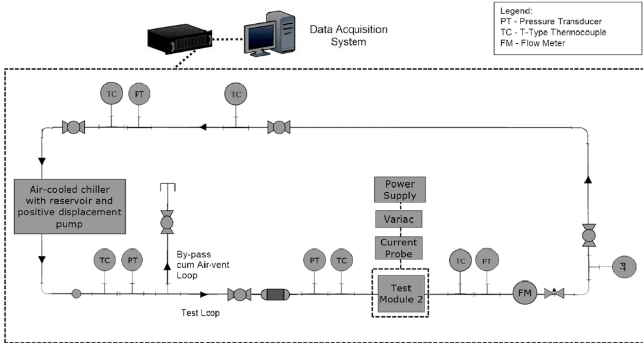
Fig. 3 Experimental test bed
