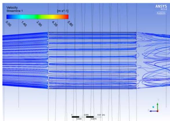
Fig. 26 Streamlines on the surface of Cfin-parallel insert
