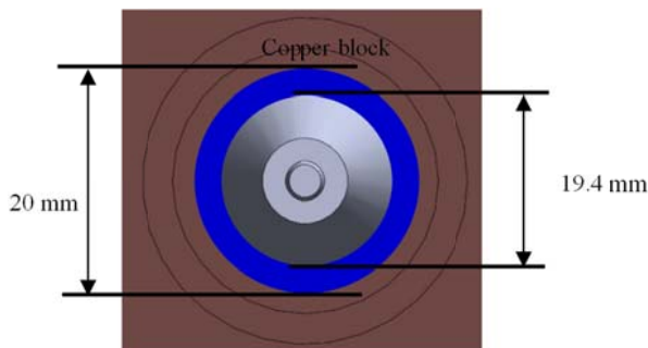
Fig. 4 Front view of the flow channel
