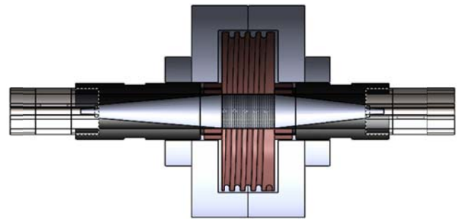
Fig. 5 Sectional view of the test module Insert design
