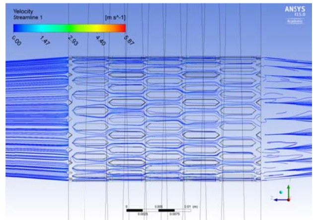
Fig. 25 Streamlines on the surface of Cfin insert
