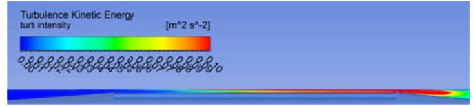
Fig. 18 Turbulence kinetic energy for Tree-parallel insert
