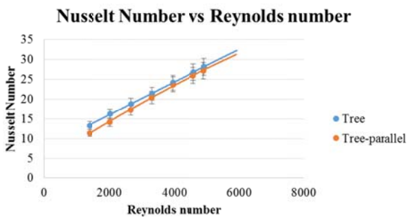
Fig. 12 Variation of Nusselt number with Reynolds number
