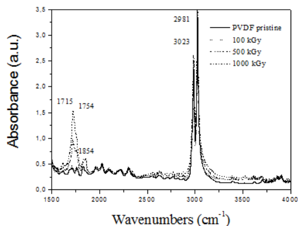
Fig. 4 FTIR spectra for pristine sample of PVDF pure and samples irradiated with 100, 500 and 1000 kGy for wavenumbers ranging from 1500 to 4000 \text{cm}^{-1}
