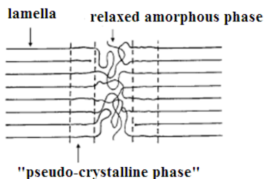
Fig. 5 The crystal / amorphous interphase [6]
