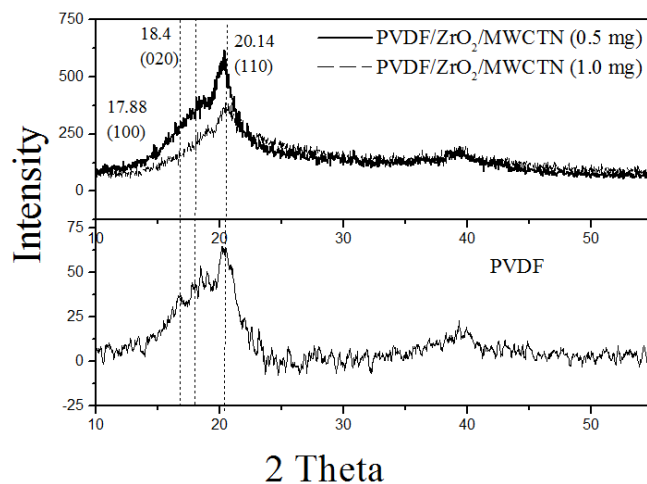
Fig. 6 X-rays diffractograms for samples of PVDF with PVDF/ZrO 2 /MWCNT (0.5 mg) and PVDF/ZrO 2 /MWCNT (1.0 mg)
