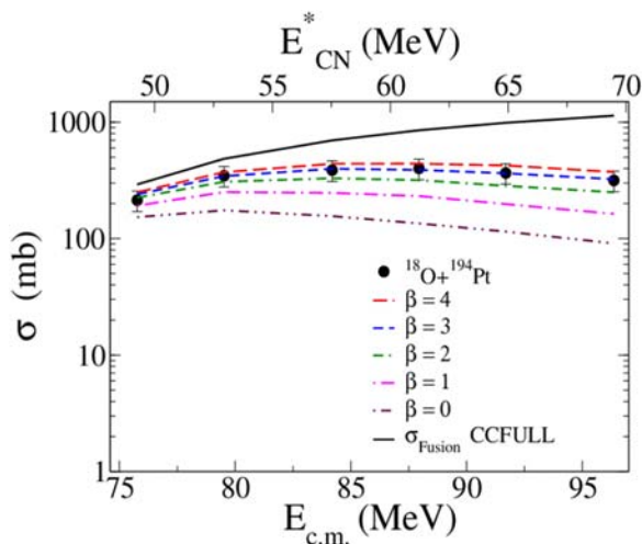
Fig. 4 The experimental ER cross section compared with model calculations assuming different \beta for the ^{18}\text{O}+^{194}\text{Pt} reaction
