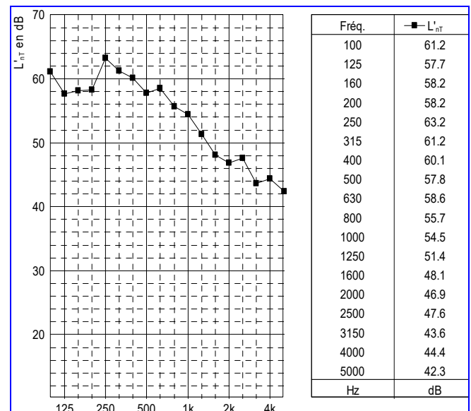
Fig. 10 Impact sound pressure level of the floor polystyrene hollow bloc, underneath layer of 16 dB acoustic reduction and then a tile covering L_{nT,w} = 57 dB
