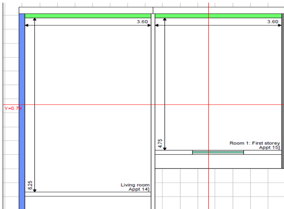
Fig. 1 Architectural sketch of the apartment under experiment
