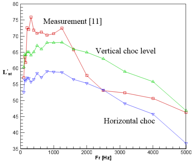
Fig. 8 Impact sound pressure level of the floor in two storey residential building in the horizontal and vertical transmission ways
