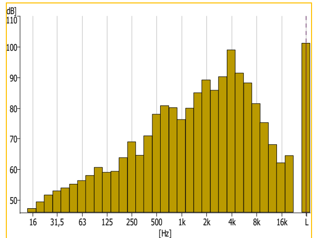
Fig. 13 Impact sound pressure level on the upper surface
