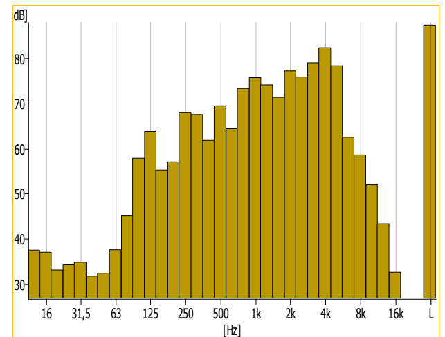
Fig. 14 Impact sound pressure level on the lower surface
