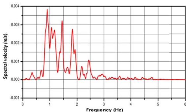
Fig. 3 Fourier spectra of velocity component
