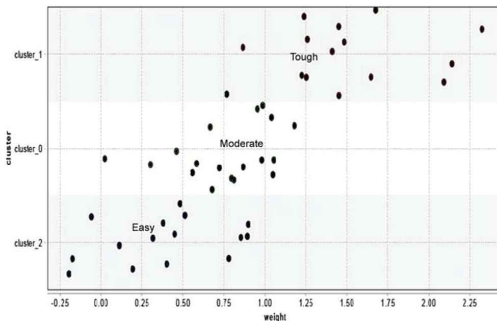
Fig. 1 Clustering
