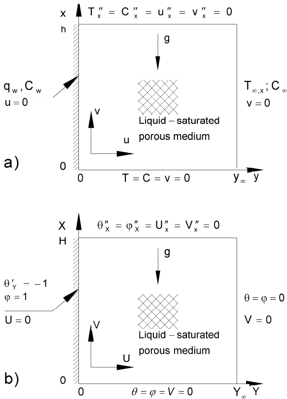
Fig. 1 (a) The vertical impermeable wall and the associated coordinate system; (b) the dimensionless domain of the problem
