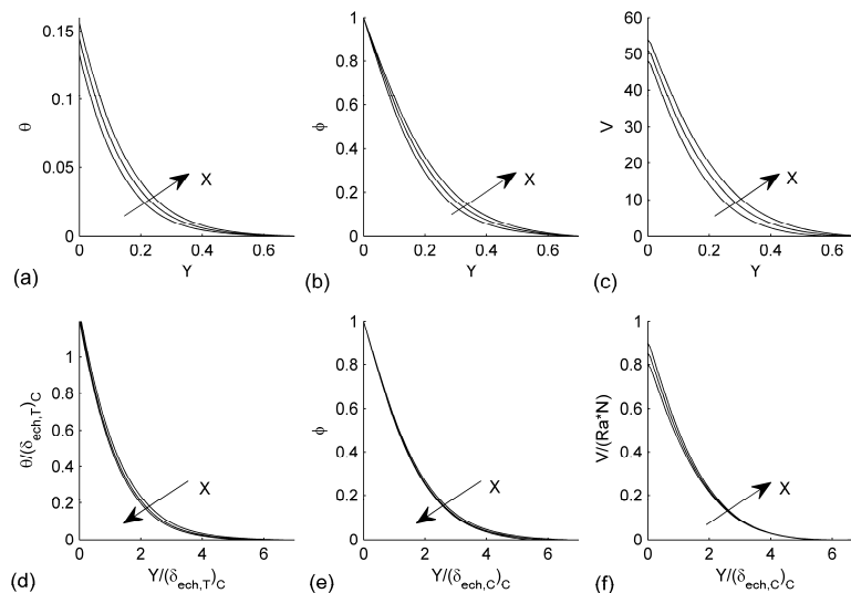
Fig. 4 (a) \theta , (b) \phi , and (c) V fields variations as a function of Y co-ordinate and the scaled (d) temperature, (e) concentration and (f) vertical velocity field variations as a function of scaled ordinate, for three abscissas: 0.63, 0.8 and 1.0, Ra = 300 , N = 0.2 , Le = 1 and S_T = 0.02
