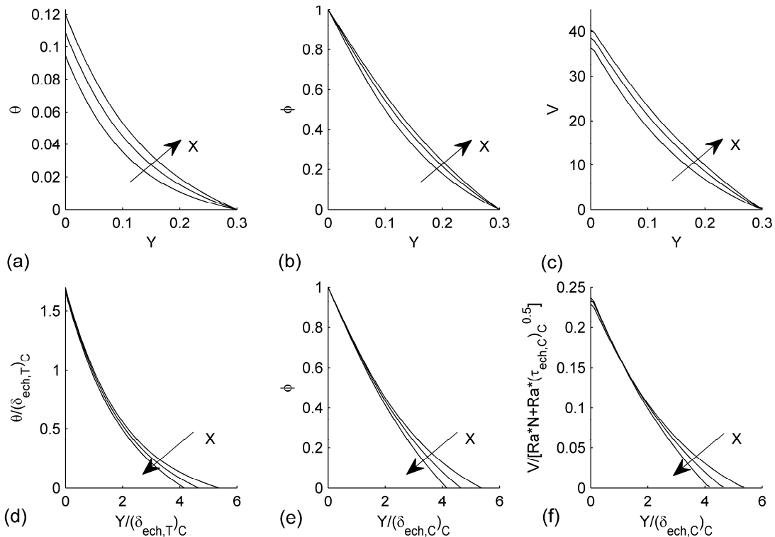
Fig. 8 (a) \theta , (b) \phi , and (c) V fields variations as a function of Y co-ordinate and the scaled (d) temperature, (e) concentration and (f) vertical velocity field variations as a function of scaled ordinate, for the abscissas: 0.50, 0.67 and 0.83, Ra = 600 , N = 0.2 , Le = 1 and S_T = 0.05
