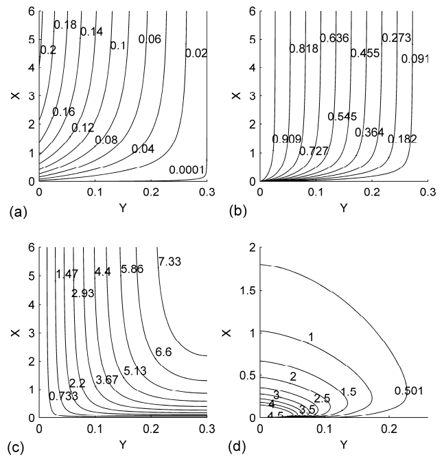
Fig. 7 (a) \theta , (b) \phi , (c) \psi , and (d) (\partial\theta/\partial X)/S_T fields. Ra = 600 , N = 0.2 , Le = 1 and S_T = 0.05
