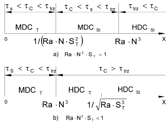
Fig. 2 The heat and mass driven natural convection regimes sequence a) Ra \cdot N^2 \cdot S_T > 1 ; b) Ra \cdot N^2 \cdot S_T < 1
