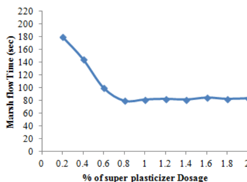
Fig. 2 Optimum Dosage of Super plasticizer for M60
