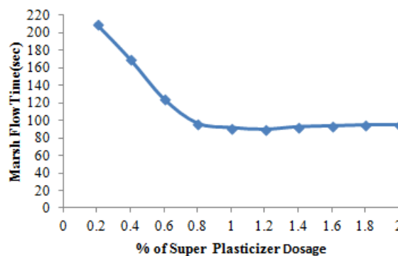
Fig. 4 Optimum Dosage of Super plasticizer for M80
