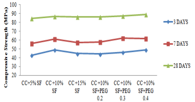
Fig. 9 Compressive Strength Result for M80
