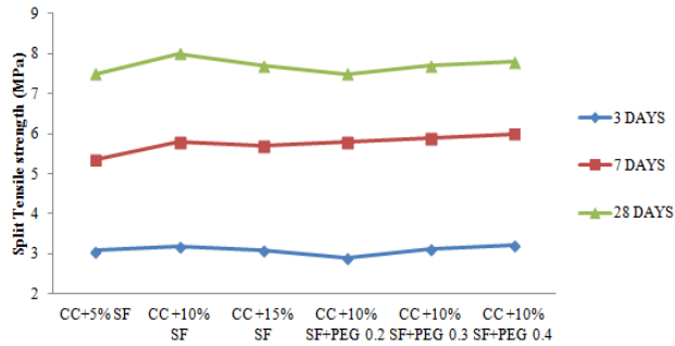
Fig. 12 Split Tensile Strength Result for M70
