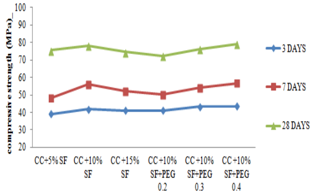
Fig. 8 Compressive Strength Result for M70
