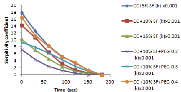
Fig. 20 Water permeability Result for M70
