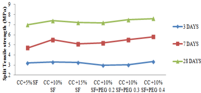
Fig. 13 Split Tensile Strength Result for M80
