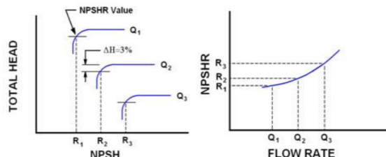
Fig. 14 NPSH R Curve [21]
