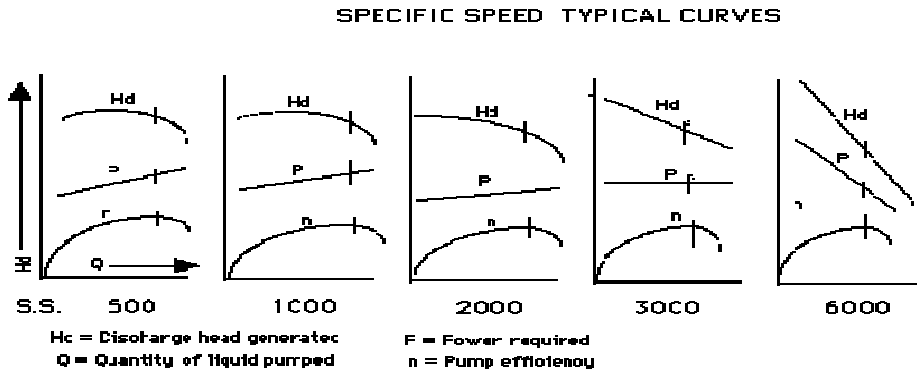
Fig. 2 Head vs. Specific Speed [10]
