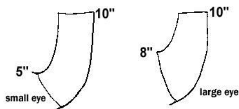
Fig. 6 Small & Large Impeller Eye [16]
