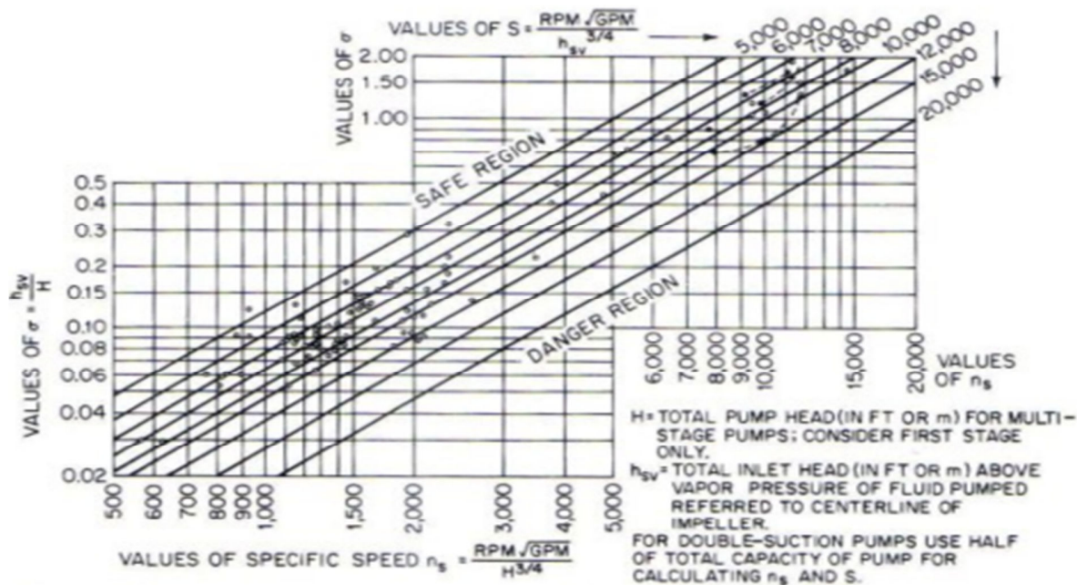
Fig. 13 Cavitation Regions [20]
