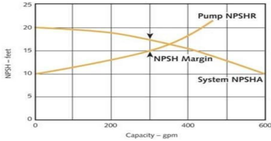
Fig. 3 NPSH Margin Ratio [13]
