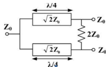
Fig. 1 Conventional Wilkinson power divider
