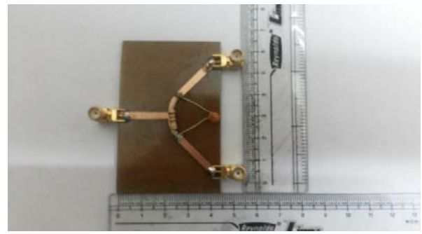
Fig. 4 Photograph of the fabricated model of the \lambda/4 transmission line Wilkinson power divider and \lambda/8 transmission line Wilkinson power divider respectively
