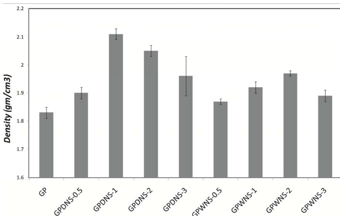
Fig. 4 Density of pure geopolymer and geopolymer nanocomposites
