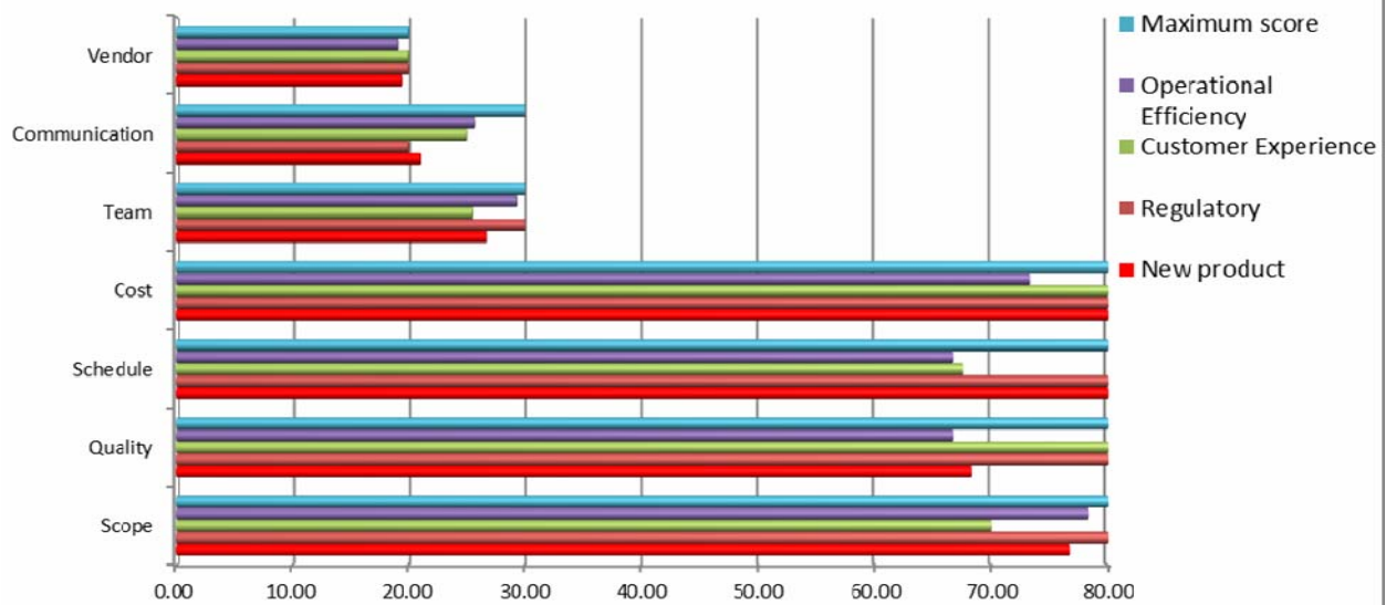
Fig. 6 Average score per attributes for each project area vs. maximum score
