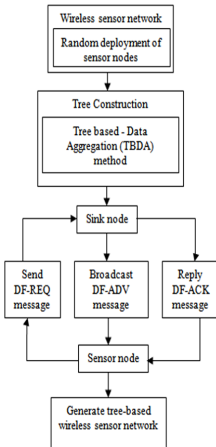
Fig. 4 Architecture of Tree based - data aggregation (TBDA) technique
