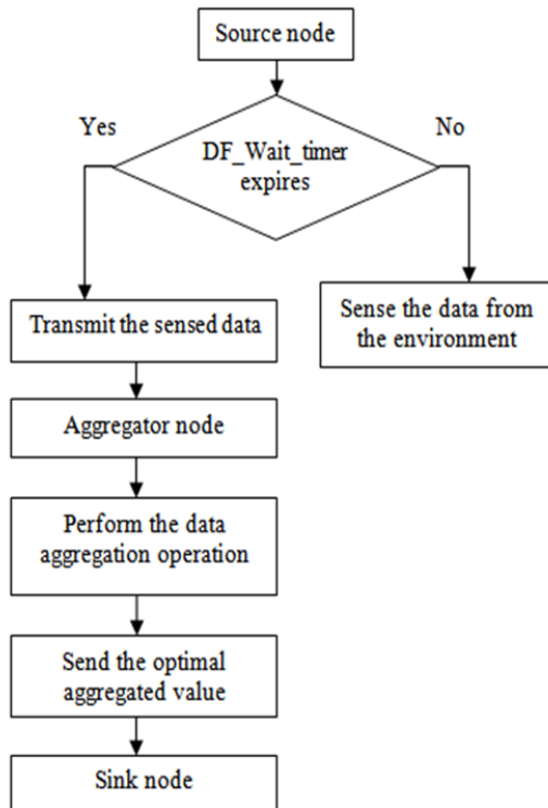
Fig. 5 Architecture of Data aggregation technique
