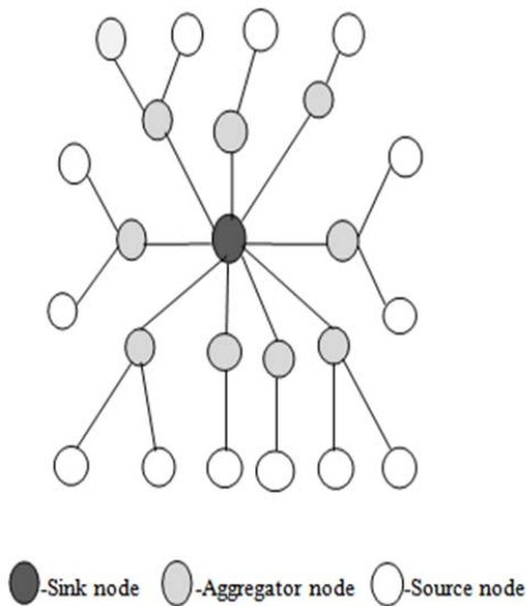
Fig. 1 Tree Topology in wireless sensor network
