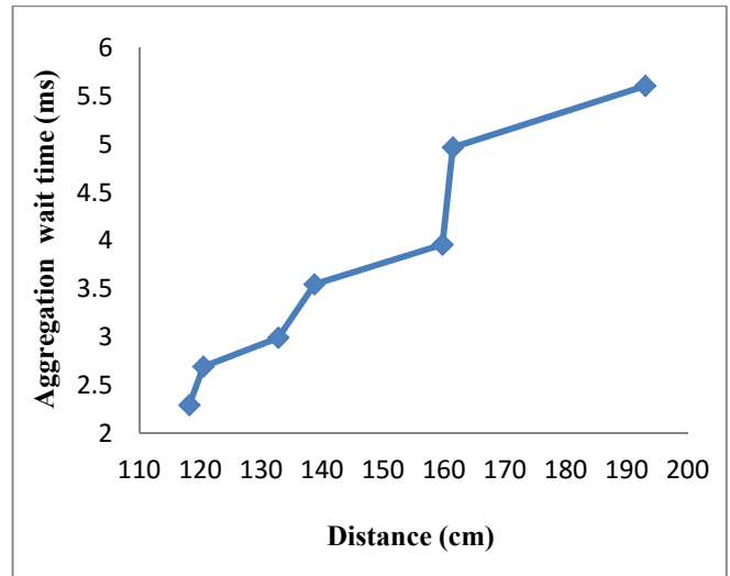
Fig. 8 Comparison of the distance and the aggregation wait time of a node by using TBDA technique
