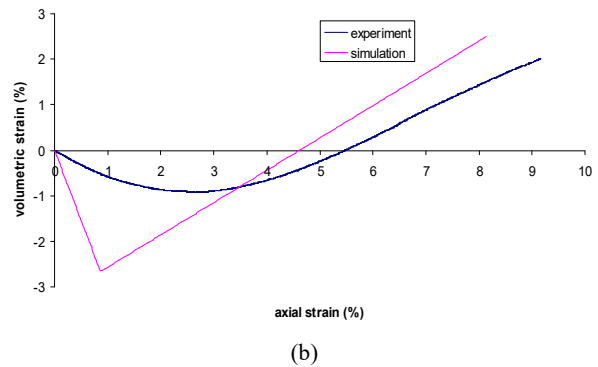
Fig. 10 (a) Evolution of the deviatoric stress in the test A4 (simulation and experiment) (b) Evolution of the volumetric strain in the test A4 (simulation and experiment)
