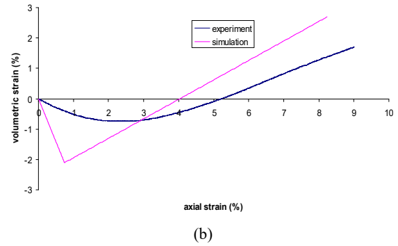
Fig. 9 (a) Evolution of the deviatoric stress in the test A3 (simulation and experiment) (b) Evolution of the volumetric strain in the test A3 (simulation and experiment)
