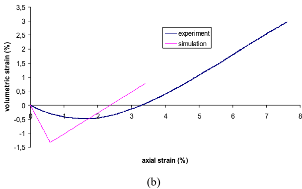
Fig. 8 (a) Evolution of the deviatoric stress in the test A2 (simulation and experiment) (b) Evolution of the volumetric strain in the test A2 (simulation and experiment)
