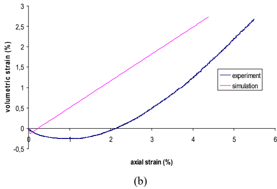
Fig. 7 (a) Evolution of the deviatoric stress in the test A1 (simulation and experiment) (b) Evolution of the volumetric strain in the test A1 (simulation and experiment)
