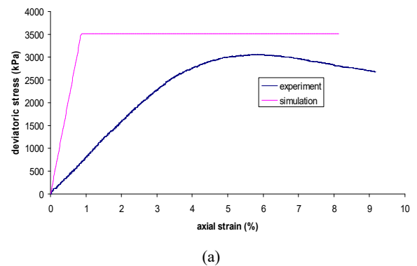
Fig. 9 (a) Evolution of the deviatoric stress in the test A3 (simulation and experiment) (b) Evolution of the volumetric strain in the test A3 (simulation and experiment)
