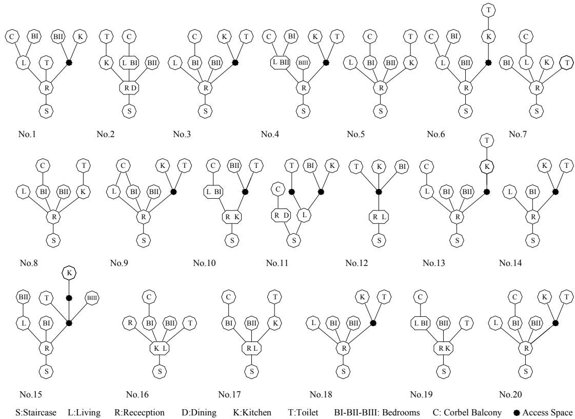
Fig. 8 Room graphs of survey buildings
