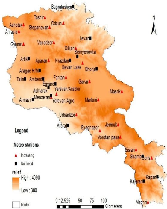
Fig. 5 Mann-Kendall test for average annual temperature over the period 1961-2012 (point data)
