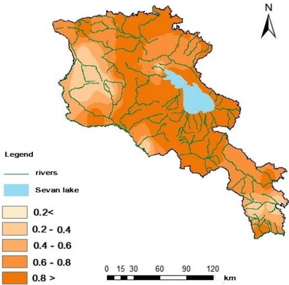
Fig. 3 Hubert segmentation tests results
