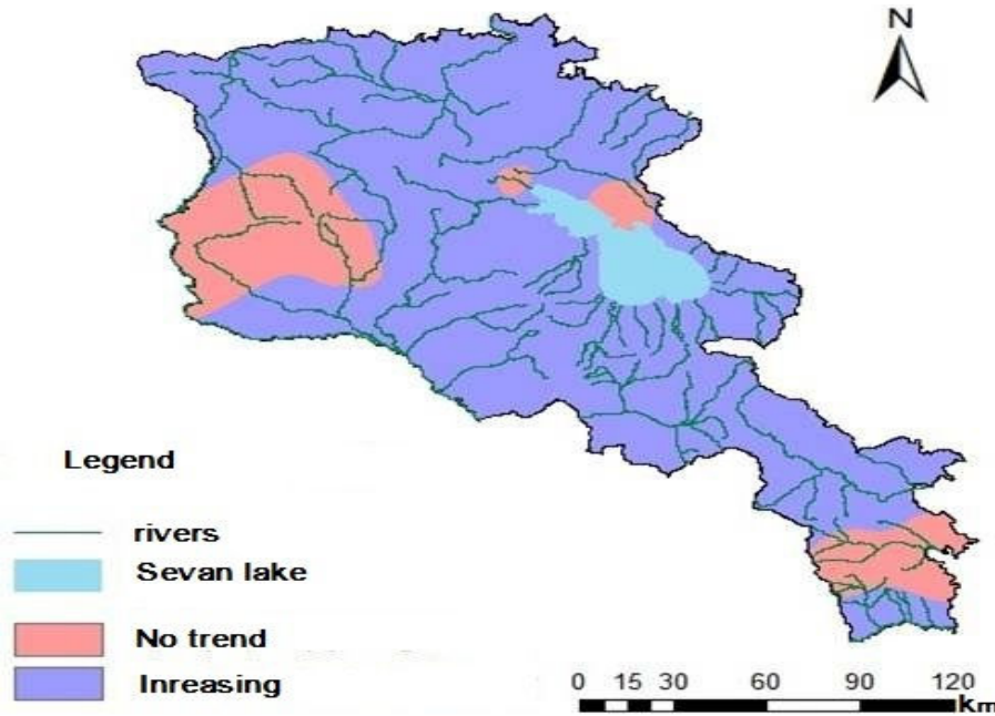
Fig. 2 Rank correlation tests results (interpolated results)
