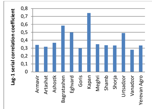
Fig. 4 Lag-1 serial correlation coefficient for the meteorological variables at the weather stations for temperature
