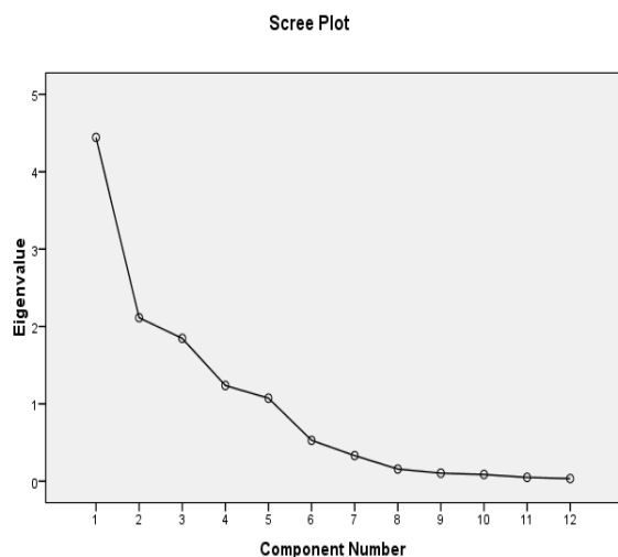
Fig. 1 Scree plot of the Eigen value
