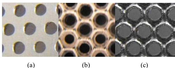
Fig. 4 Photo of accelerator grid downstream surface erosion; (a) new grid, (b) after 200h operating, (c) after 3700h operating
