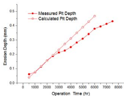
Fig. 6 Accel grid pit erosion comparison
