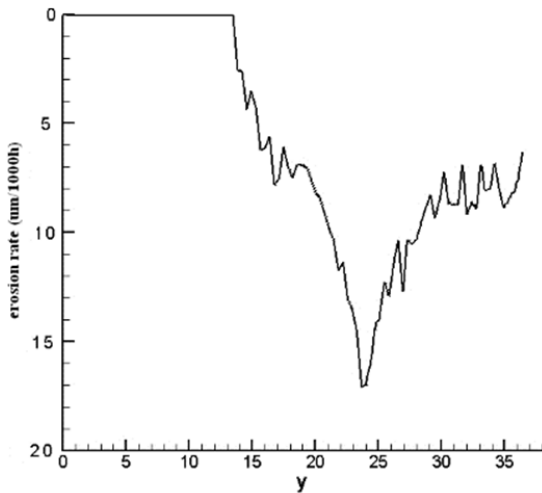
Fig. 2 Section of pit erosion rate
