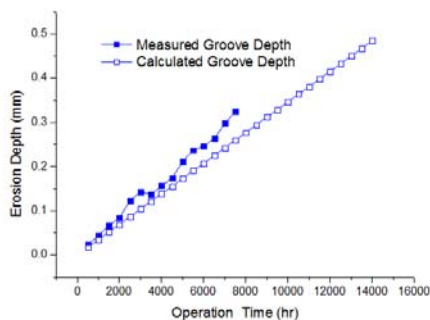
Fig. 7 Accel grid groove erosion comparison
