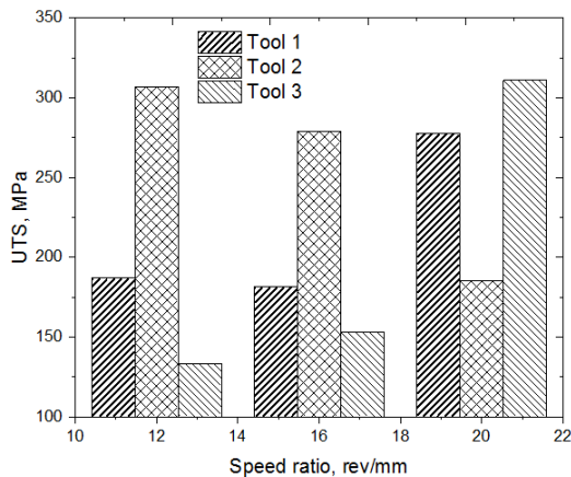
Fig. 8 UTS vs speed ratio for the tools used
