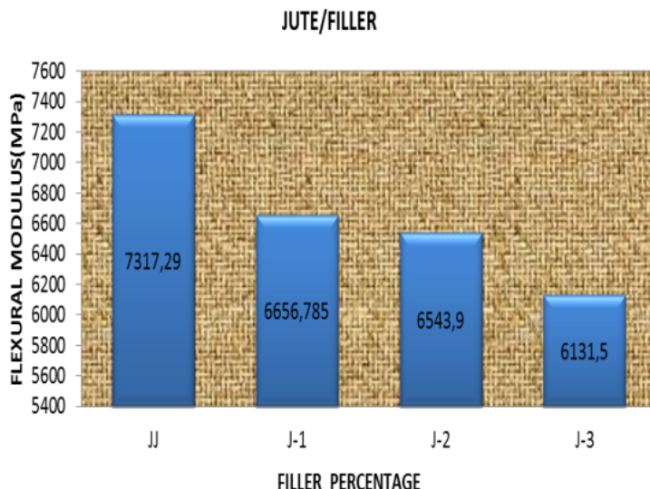
Fig. 5 Flexural Modulus of Composites in various stages of filler addition
