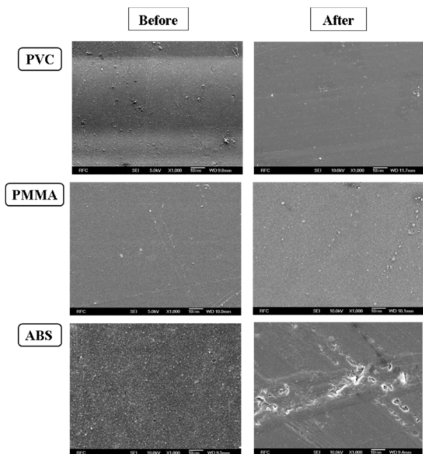
Fig. 2 SEM images of plastics before and after the mild heat treatment at 100°C for 60 sec
