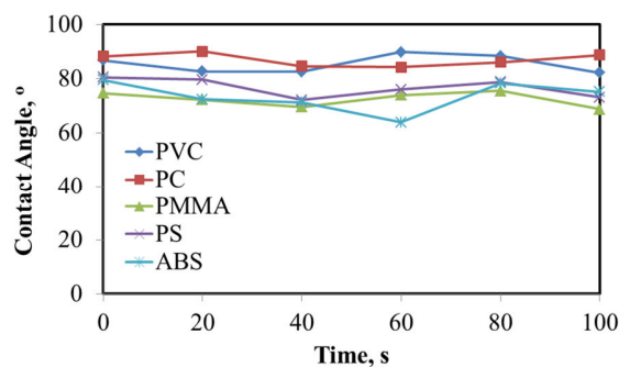
Fig. 1 Contact angle changes in the plastic surfaces before and after mild heat treatment at various times
