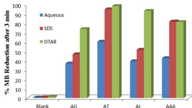
Fig. 5 MB reduction % with ANP as catalyst in aqueous, SDS and DTAB micellar medium at 298.15 K, after 3 min
