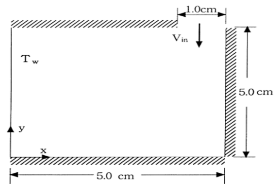
Fig. 2 Cube mold cavity [1]
