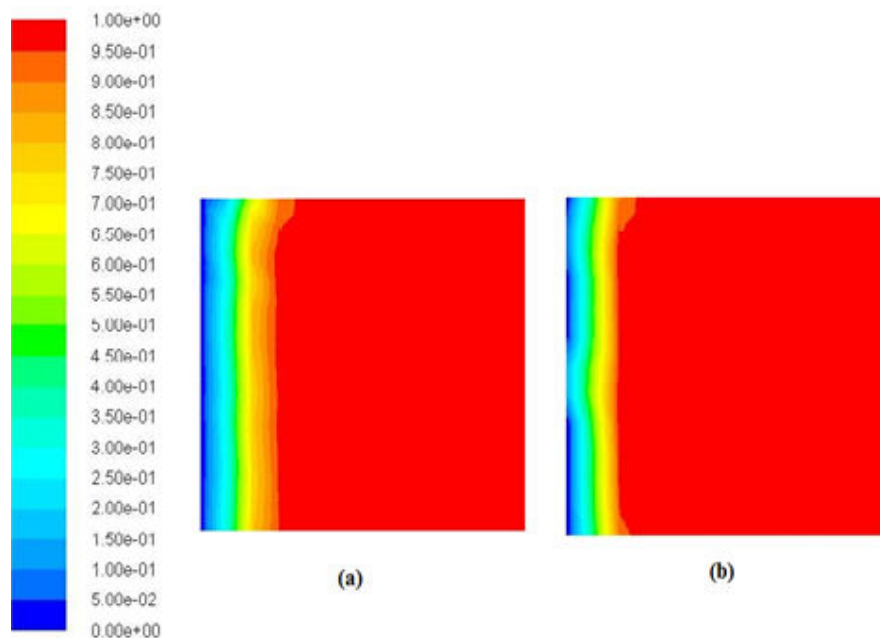
Fig. 8 Liquid fraction contour at different inlet velocity for t = 10 sec, T_i = 973 K, T_{wl} = 773 K, h_g = 5 cm and filling at the right side of the top plane (a) v = 0.1 m/s and (b) v = 0.2 m/s
