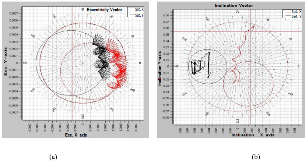
Fig. 8 (a) Satellite X, Y eccentricity evolution for 3 months (b) Satellite X, Y inclination evolution for 3 months
