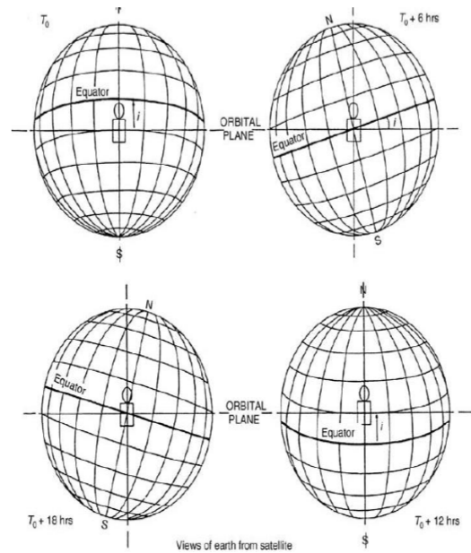
Fig. 5 Satellite inclination-induced Yaw Variation along the orbit
