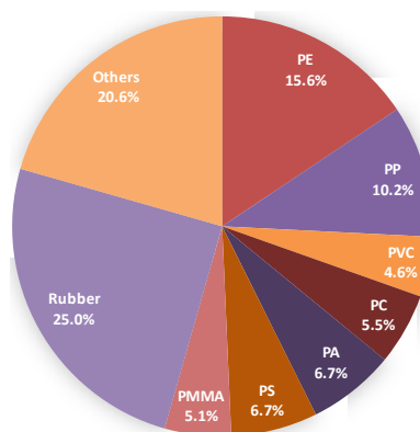
Fig. 2 Quantified polymer compositions in ASR
