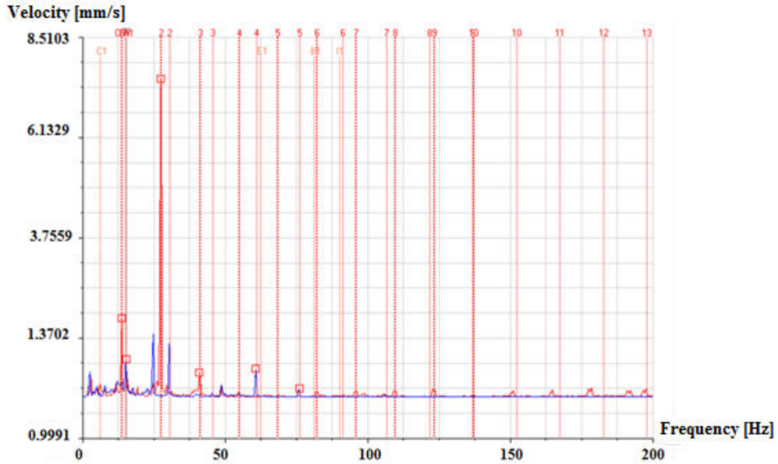
Fig. 6 Spectral Image superimposed on bearing N°02 RH
