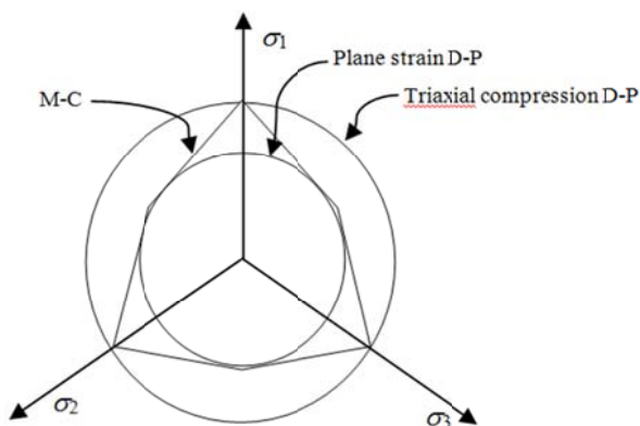
Fig. 8 Matching of Drucker-Prager and Mohr-Coulomb criteria
