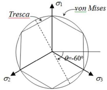
Fig. 3 Comparison between Tresca and von Mises at uniaxial compression
