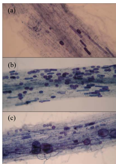
Fig. 2 Stained roots colonization of Lactuca sativa by arbuscular mycorrhizal fungi (AMF), (a) Control sample with low AMF colonization, (b) Sample amended with “NovaFerm” inoculum (arbuscules), (c) The same sample colonized by arbuscules, vesicles, extra and intraradical hyphae
